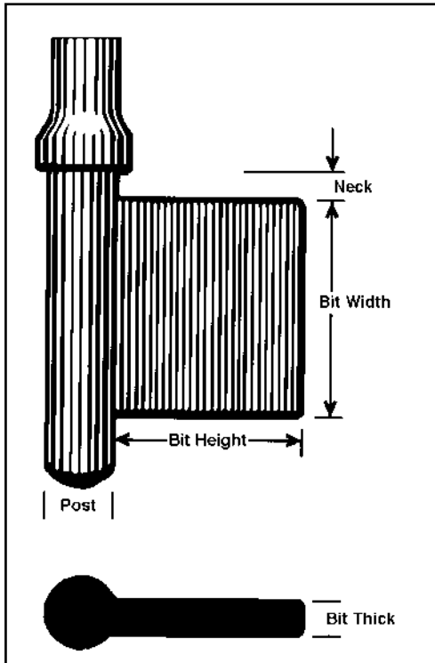
Dimensions of a Bit Key
